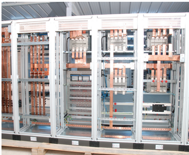
Project: Export of Electrical Panels for the Metro B Station (Lyon - France) Year: 2012
